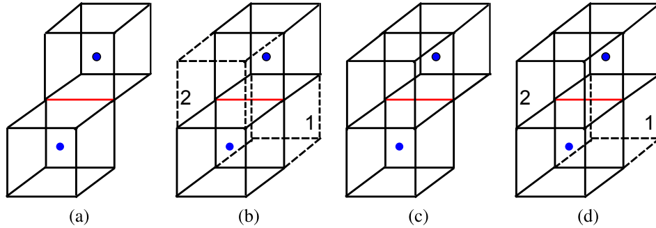
Fig. 6. Partition mesh non-manifold edge detection and cure. (a) The red edge is a non-manifold edge. (b) All the neighboring voxels. (c) After addition of the upper left voxel 2, the red edge becomes a manifold edge. (d) Neighborhood status after cure.
