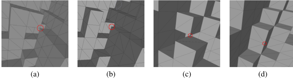
Fig. 5. Partition mesh non-manifold vertex detection and cure applied to the brain Brodmann area region 16 data. (a) and (c) The vertices in the red circles are non-manifold vertices that were detected. (b) and (d) The vertices in the red circles are manifold vertices after cure.
